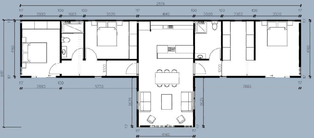
FLOOR PLAN - 109 sqm
